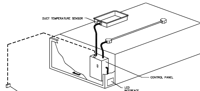
TYPICAL HOOD CONTROL PANEL INSTALLATION
