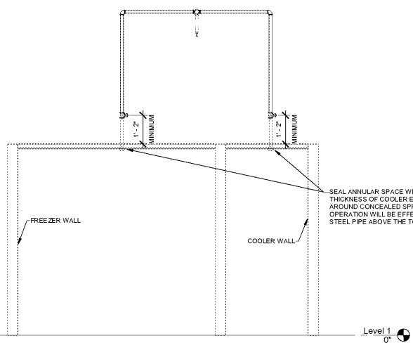
2 WALK-IN FREEZER/COOLER INSTALLATION DETAIL 1/2" = 1'-0"
