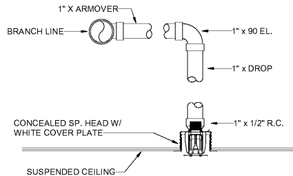
3 TYPICAL RECESSED PENDENT SPRINKLER NOT TO SCALE
