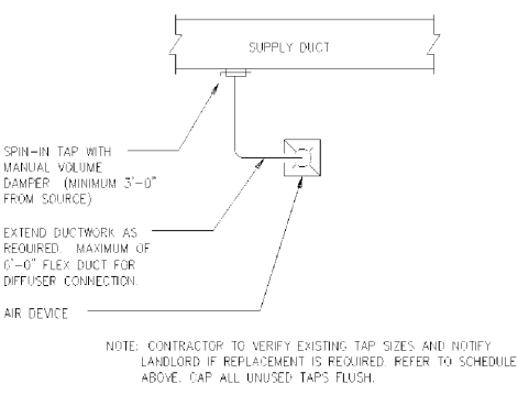
04 DIFFUSER CONNECTION SCALE = NONE
