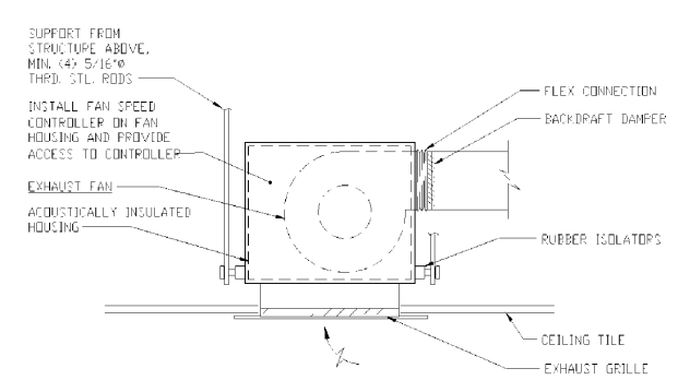
07 INLINE EXHAUST FAN DETAIL SCALE = NONE
