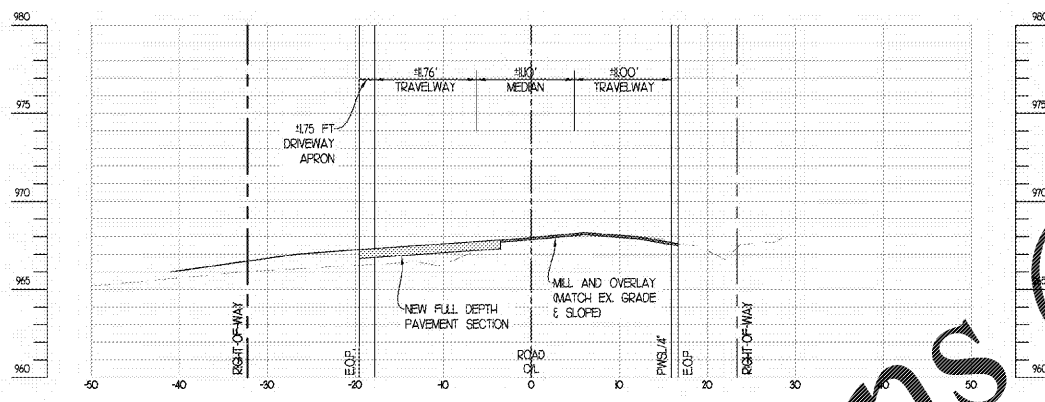
STATION: 5+00
