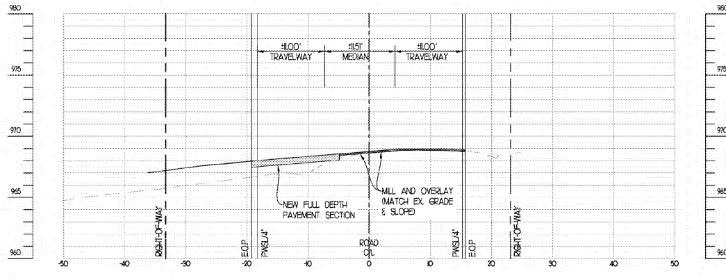
STATION: 4+00
