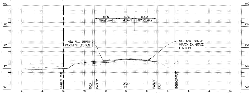
STATION: 6+00
