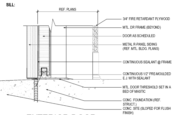
EXTERIOR DOOR 3'-1"
