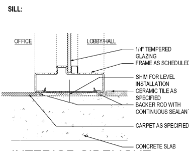
INTERIOR SIDELIGHT 3'-1"
