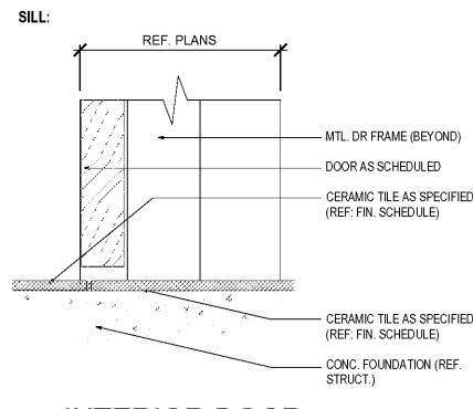
INTERIOR DOOR 3'-1"
