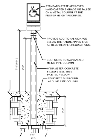
A.D.A. SIGN DETAIL SCALE: NOT TO SCALE
