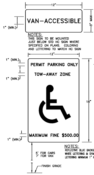
A.D.A. PARKING SIGN DETAIL SCALE: NOT TO SCALE
