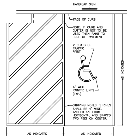
A.D.A. STRIPING DETAIL SCALE: NOT TO SCALE
