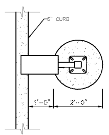
15' AREA LIGHT PLAN VIEW NTS
