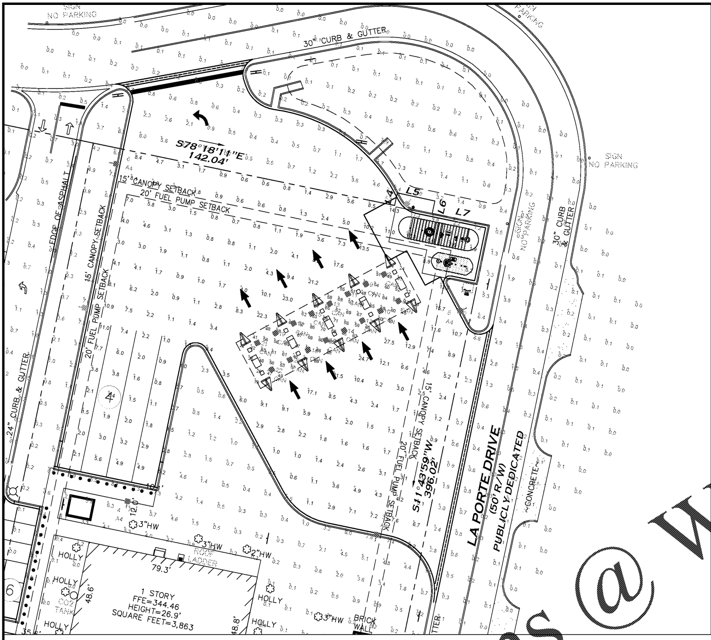
PARTIAL PHOTOMETRIC SITE PLAN
