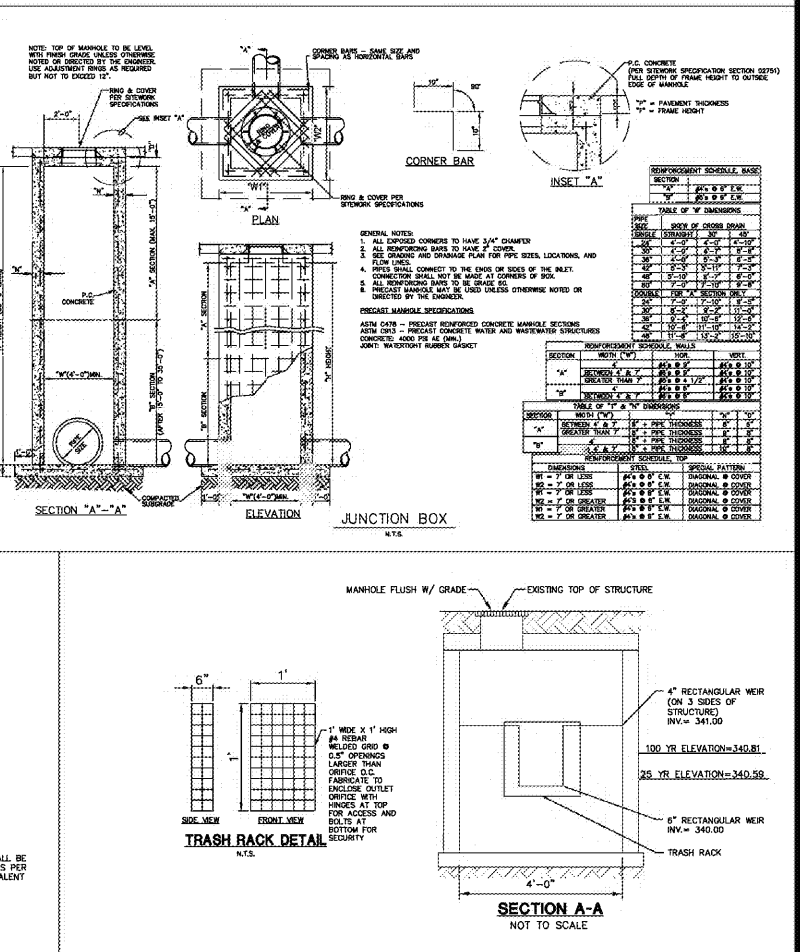
PRECAST MANHOLE JUNCTION BOX
