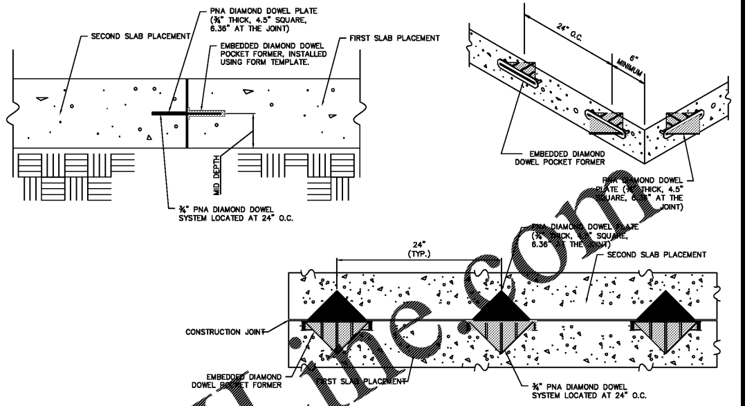
PNA DIAMOND DOWEL SYSTEM DETAILS (FOR ALTERNATE TO SMOOTH DOWEL SHOWN IN JOINTING DETAILS)
