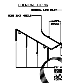
9 ANSUL FIRE SUPPRESSION ISOMETRIC DETAIL 2 SCALE: NO SCALE
