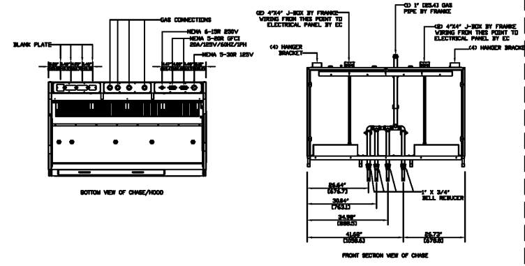
5 UTILITY DETAILS 2 SCALE: NO SCALE
