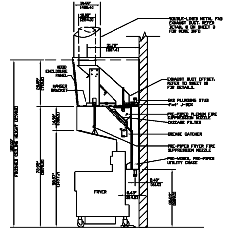
2 FRYER HOOD SECTION VIEW 2 SCALE: NO SCALE
