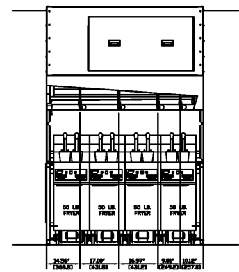
1 ANSUL FIRE SUPPRESSION PIPING DETAIL - OPTIONAL FRYER CONFIGURATION 2 SCALE: NO SCALE
