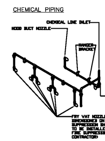
8 AMEREX FIRE SUPPRESSION ISOMETRIC DETAIL 2 SCALE: NO SCALE
