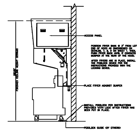
3 FRYER HOOD RIGHT END VIEW 2 SCALE: NO SCALE
