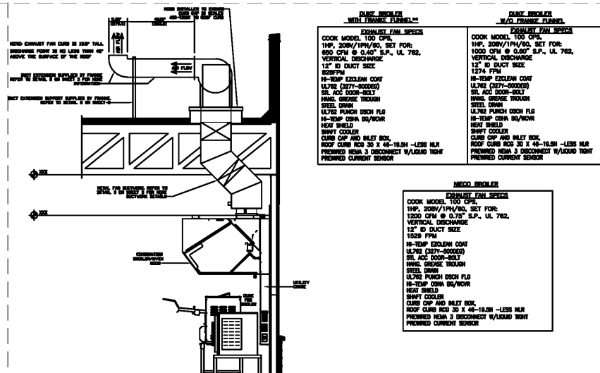
9 EXHAUST FAN DETAIL SCALE: NO SCALE
