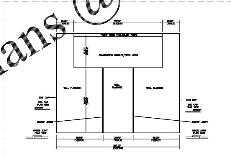
8 WALL FLASHING DETAIL SCALE: NO SCALE
