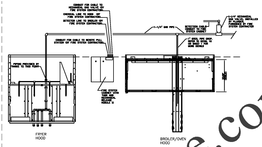
3 TYPICAL WALL MOUNTED FIRE SYSTEM USING ONE SYSTEM FOR TWO HOODS SCALE: NO SCALE
