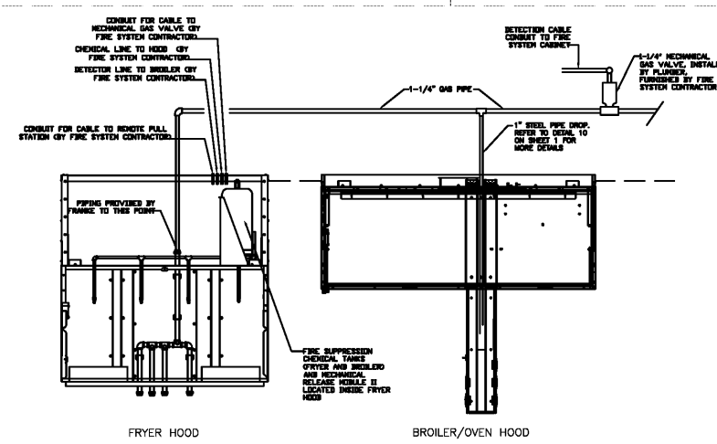
1 FIRE SUPPRESSION PIPING DETAIL SCALE: NO SCALE
