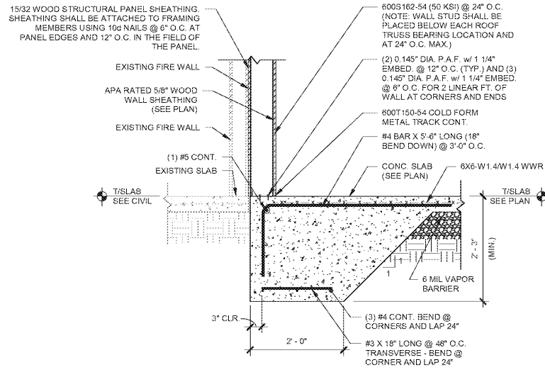
1 TYP. FOOTING DETAIL 2 S3.2 3/4" = 1'-0"
