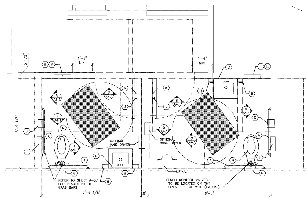
1 RESTROOMS ENLARGED PLAN A4.1 SCALE: 1/2" = 1'-0"
