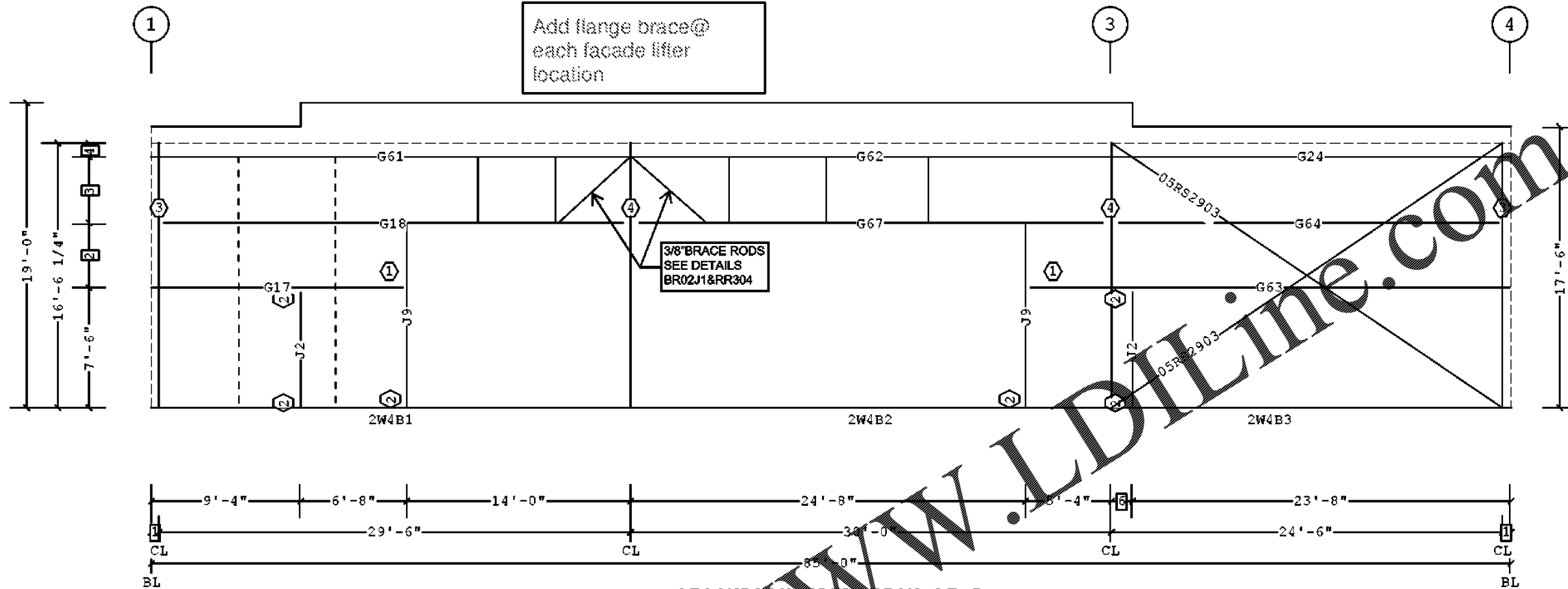
SECONDARY ELEVATION AT D
