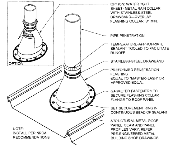
11 VENT THRU ROOF DETAIL A4.2 NOT TO SCALE
