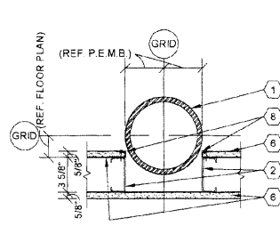
3 COLUMN DETAIL A4.2 SCALE: 1 1/2" = 1'-0"
