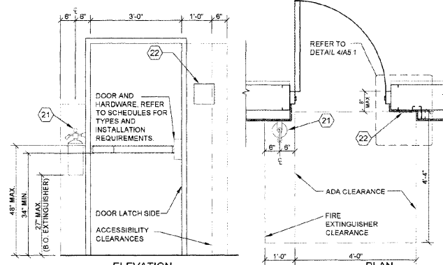
10 FIRE EXTINGUISHER DETAIL A4.2 SCALE: 1/2" = 1'-0"
