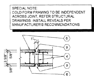
2 GYPSUM BOARD C.J. DETAIL A4.2 SCALE: 1 1/2" = 1'-0"
