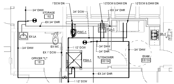
2 ENLARGED FIRST FL PL - DOM - AREA A - EXAM/TL/SHWR P2.1.3/P4.1.4 1/4" = 1'-0"
