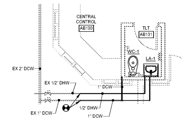
3 ENLARGED FIRST FL PL - DOM - AREA A - CENTRAL CTRL TLT P2.1.3/P4.1.4 1/4" = 1'-0"
