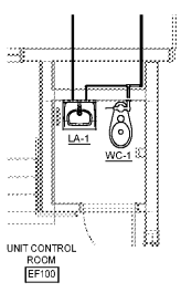
5 ENLARGED FIRST FL PL - DOM - AREA B - UNIT CTRL RM TLT P2.1.4/P4.1.4 1/4" = 1'-0"
