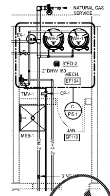
4 ENLARGED FIRST FL PL - DOM - AREA B - MECH P2.1.4/P4.1.4 1/4" = 1'-0"
