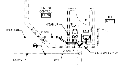
3 ENLARGED FIRST FL PL - SAN - AREA A - CENTRAL CTRL TLT P2.1.1/P4.1.1 1/4" = 1'-0"
