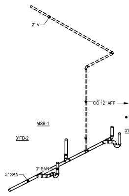
S5 SAN RISER - MECH/ELEC/JAN NO SCALE
