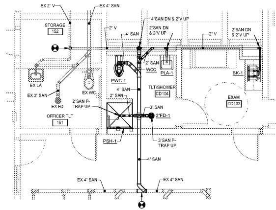
2 ENLARGED FIRST FL PL - SAN - AREA A - EXAM/TLT/SHWR P2.1.1/P4.1.1 1/4" = 1'-0"
