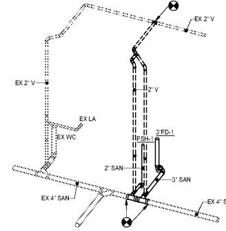
S1 SAN RISER - SHWR RM NO SCALE
