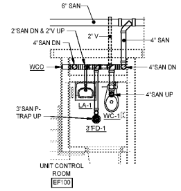
6 ENLARGED FIRST FL PL - SAN - AREA B - UNIT CTRL RM TLT P2.1.2/P4.1.1 1/4" = 1'-0"
