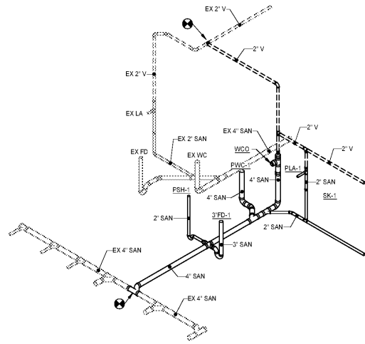
S2 SAN RISER - EXAM/TLT/SHWR NO SCALE
