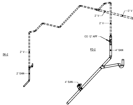
S4 SAN RISER - LAUNDRY NO SCALE
