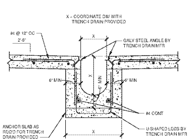
TRENCH DRAIN DETAIL
