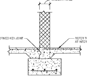
SECTION AT INTERIOR DOORS
