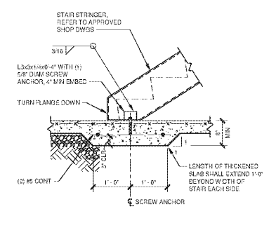
STAIR
