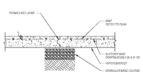
CONSTRUCTION JOINT
