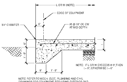
EXTERIOR EQUIPMENT PAD
