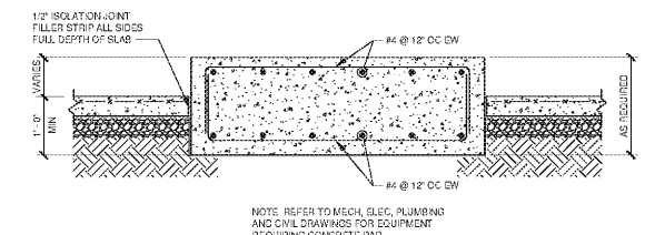
HEAVY EQUIPMENT PAD
