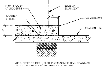
HOUSEKEEPING PAD
