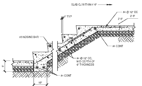
INTERIOR CONCRETE STAIR DETAIL
