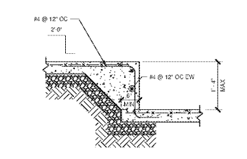
STEP IN SLAB ON GRADE
