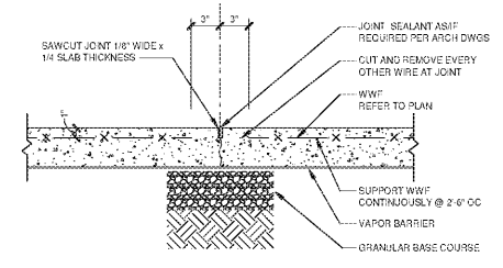
CONTROL JOINT
