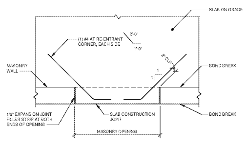
PLAN AT INTERIOR DOORS
