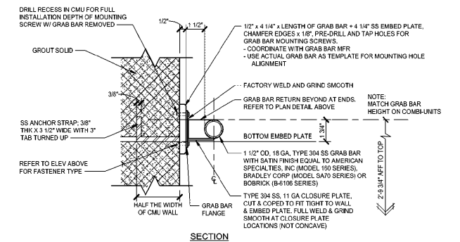
1 TYP A7.4.2 REMOVABLE GRAB BAR W/ CONTINUOUS EMBED PLATE DETAIL 3" = 1'-0"
