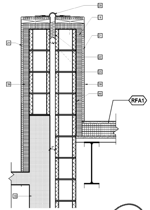
6 SECTION DETAIL A5.1.2/A5.2.1 1 1/2" = 1'-0"
