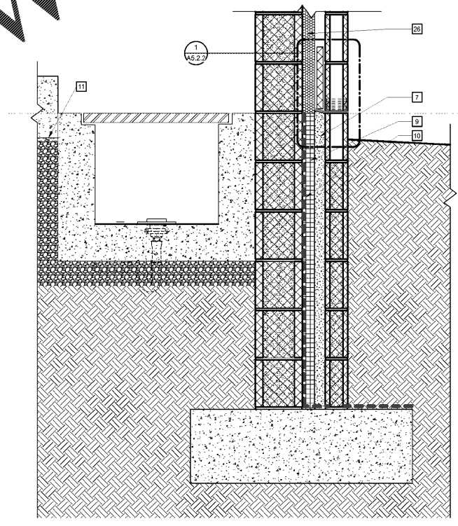
3 SECTION DETAIL A5.1.1/A5.2.1 1 1/2" = 1'-0"
