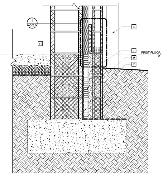
1 SECTION DETAIL A5.1.1/A5.2.1 1 1/2" = 1'-0"
