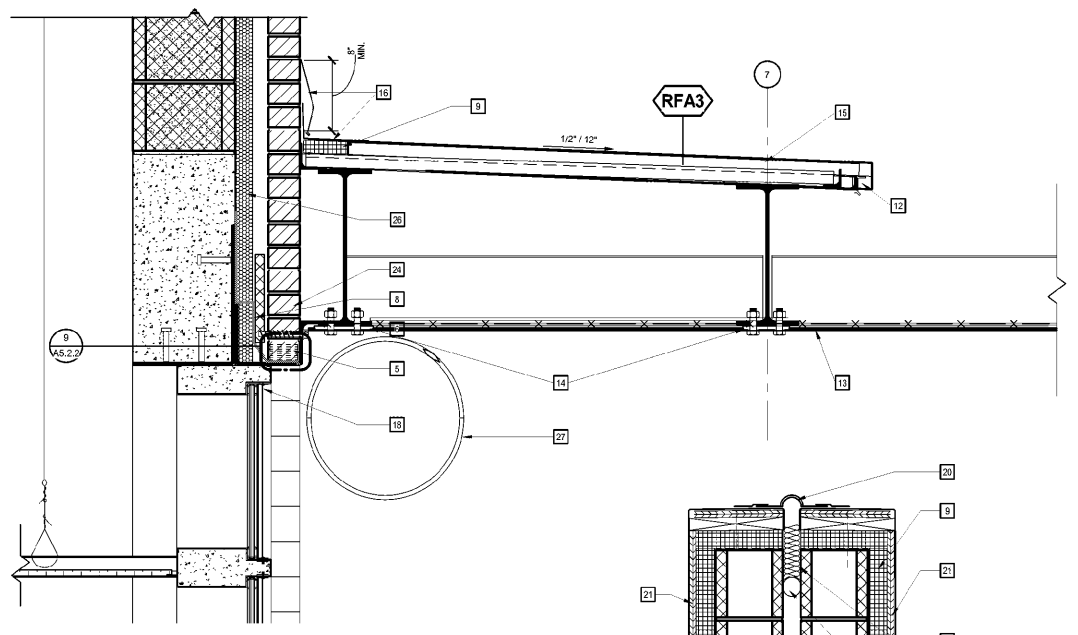
9 SECTION DETAIL A5.1.2/A5.2.1 1 1/2" = 1'-0"
