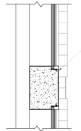
8 SECTION DETAIL A5.1.2/A5.2.1 1 1/2" = 1'-0"
