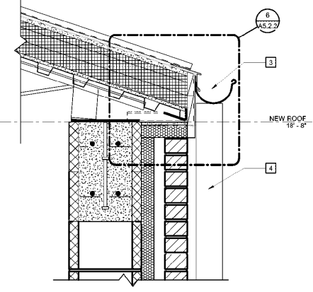
2 SECTION DETAIL A5.1.1/A5.2.1 1 1/2" = 1'-0"
