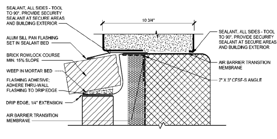
7 EXT DETENTION WINDOW SILL DETAIL TYP A3.4.1 3" = 1'-0"
