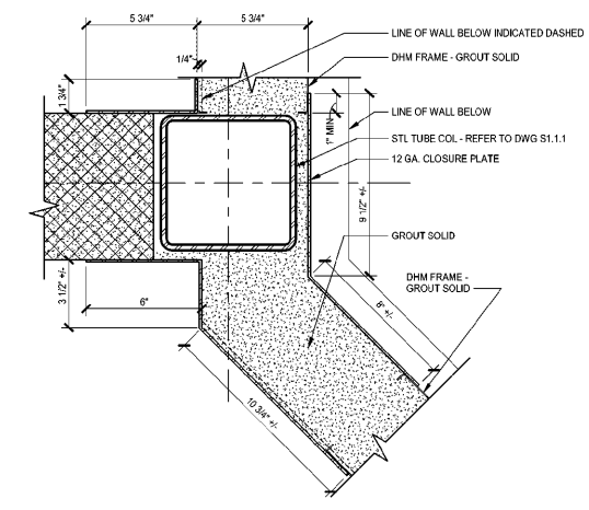
8 PLAN DETAIL - CONTROL RM WINDOWS/ COL TYP A3.4.1 3" = 1'-0"
