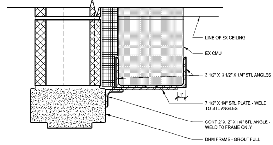
11 HEAD AT DOOR DEF111 TYP A3.4.1 3" = 1'-0"
