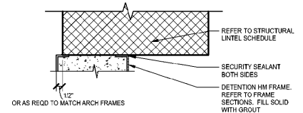
10 HEAD DETAIL - INSET TYP A3.4.1 3" = 1'-0"
