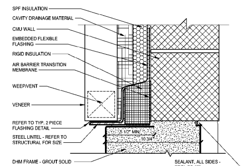
4 HEAD DETAIL TYP A3.4.1 3" = 1'-0"
