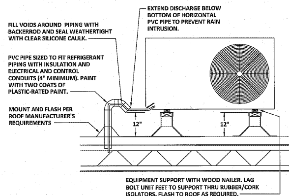
2 SECTION @ OUTDOOR UNIT ON ROOF M3.1 NOT TO SCALE
