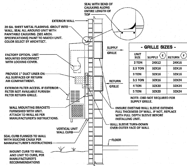
1 WALL MOUNTED HEAT PUMP W/CURB DETAIL M3.1 NOT TO SCALE
