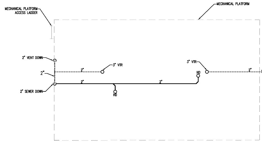
1 MECHANICAL PLATFORM PLUMBING PLAN SCALE: 1/4"=1'-0"
