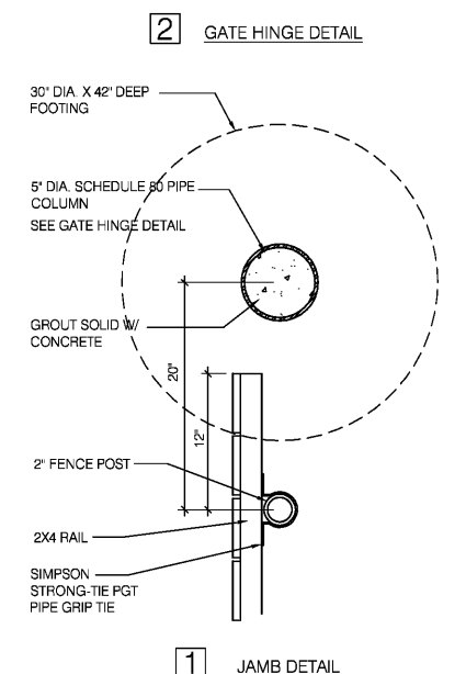
GATE DETAILS VARIES C
