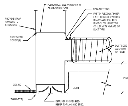
3 LINEAR SLOT DIFFUSER DETAIL M-2.1 NOT TO SCALE
