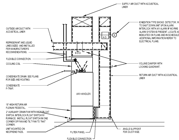
7 AIR HANDLER DETAIL M-2.1 NOT TO SCALE
