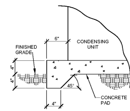
10 CONDENSING UNIT PAD DETAIL M-2.1 NOT TO SCALE
