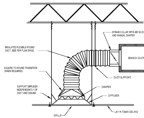
1 LAY-IN AIR DEVICE INSTALLATION DETAIL M-2.1 NOT TO SCALE
