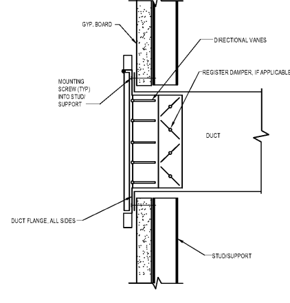
2 WALL MOUNTED AIR DEVICE DETAIL M-2.1 NOT TO SCALE
