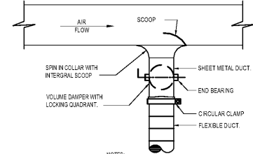
6 TYPICAL BRANCH TAKE-OFF DETAIL M-2.1 NOT TO SCALE
