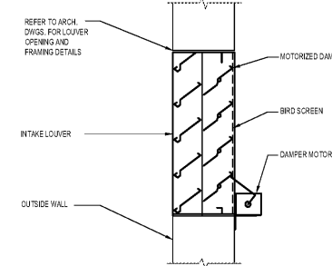
13 COMBINATION LOUVER DETAIL M-2.1 NOT TO SCALE
