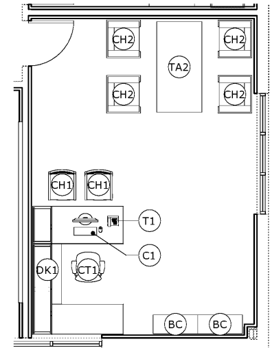
3 TYPICAL OFFICE, TYPE 2 SCALE: 1/4" = 1'-0"
