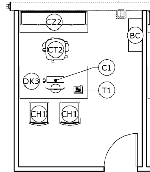
2 TYPICAL OFFICE, TYPE 1 SCALE: 1/4" = 1'-0"
