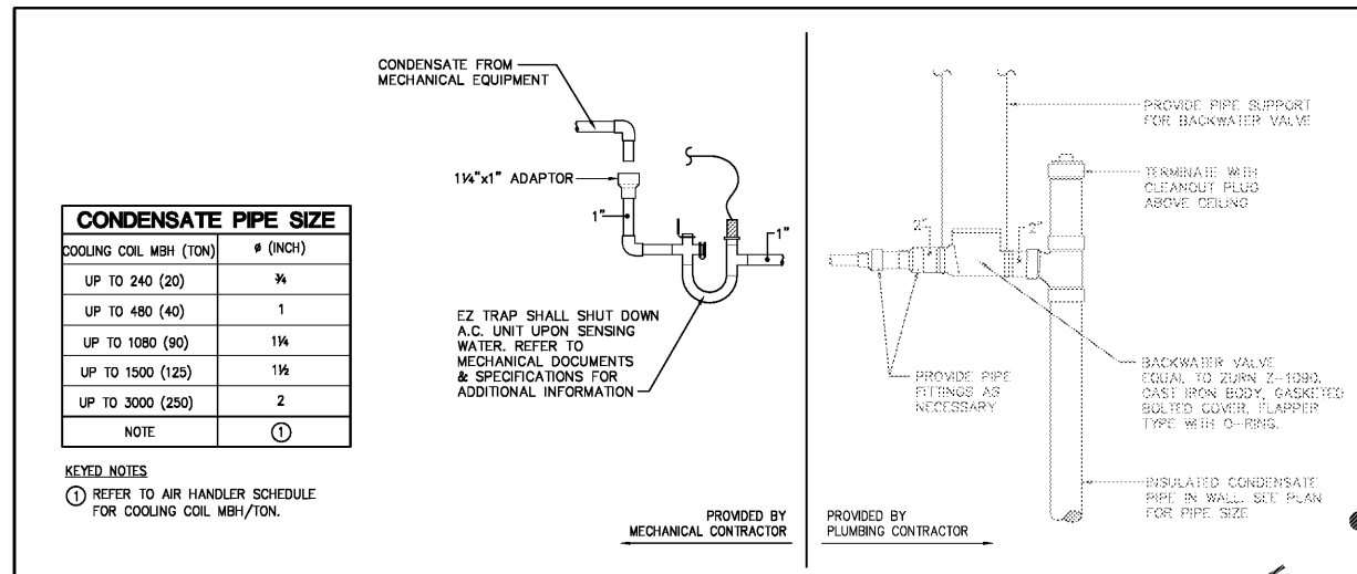
CEILING HUNG AIR HANDLER CONDENSATE DRAIN AND TRAP DETAIL NO SCALE. TYP. OF AH-1-1 & QAH 1-1X
