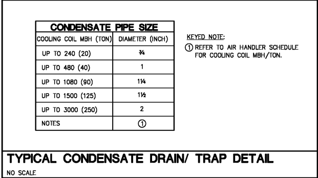
TYPICAL CONDENSATE DRAIN/ TRAP DETAIL NO SCALE.
