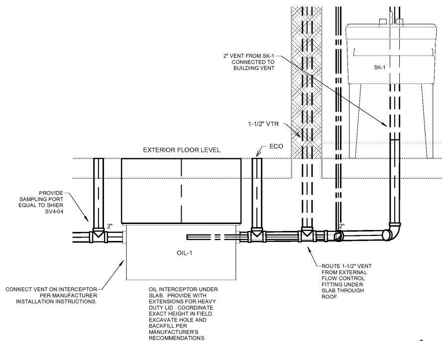
6 OIL INTERCEPTOR DETAIL SV-P3.01 1" = 1'-0"
