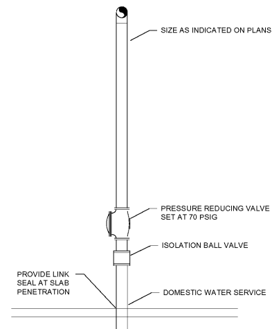
5 DOMESTIC WATER ENTRANCE DETAIL P3.01 NO SCALE
