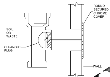
4 WALL CLEANOUT P3.01 NO SCALE
