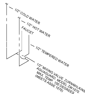
3 TYPICAL LAVATORY MIXING VALVE P3.01 SCALE: NONE
