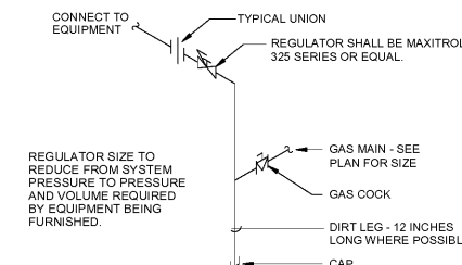
1 TYPICAL GAS CONNECTION P3.01 NO SCALE
