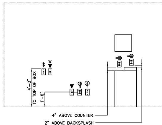
DETAIL TYPICAL MOUNTING HEIGHTS NOT TO SCALE
