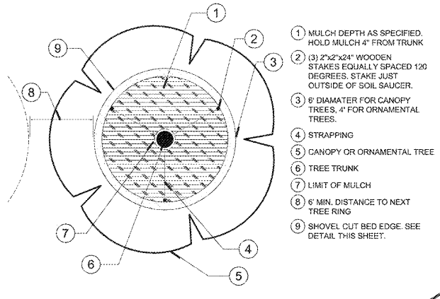
3 MULCHING RING AT TREES N.T.S. DDG-GE-LA-02
