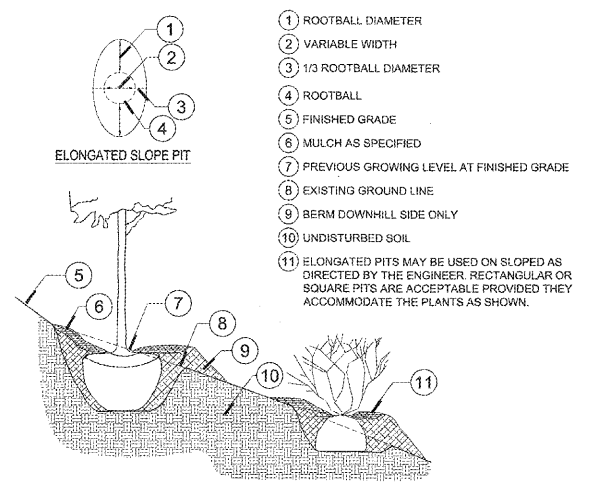
5 PLANT PLACEMENT ON SLOPE N.T.S. DDG-GE-LA-06
