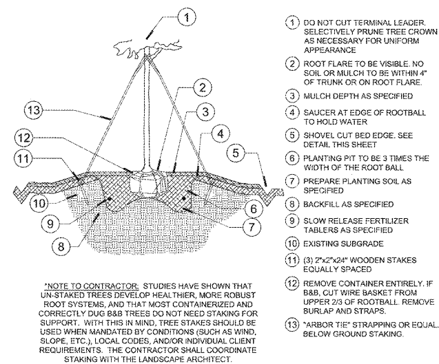
1 STAKED TREE (TYPICAL) N.T.S. DDG-GE-LA-01
