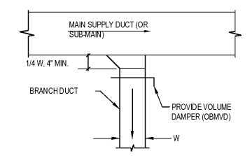
SUPPLY AIR DUCT
