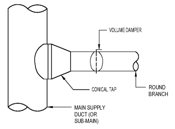
SUPPLY AIR DUCT
