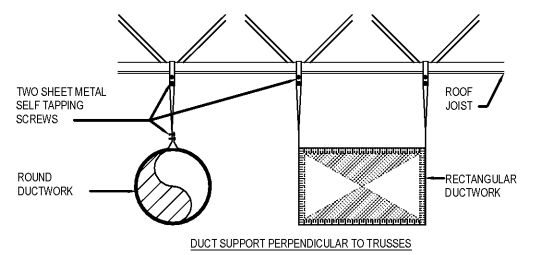
3 DUCT HANGER DETAILS M-4 SCALE: NTS
