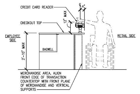
3 ADA FRONT CHECKOUT COUNTER SECTION A6 SCALE: 1/2" = 1'-0"
