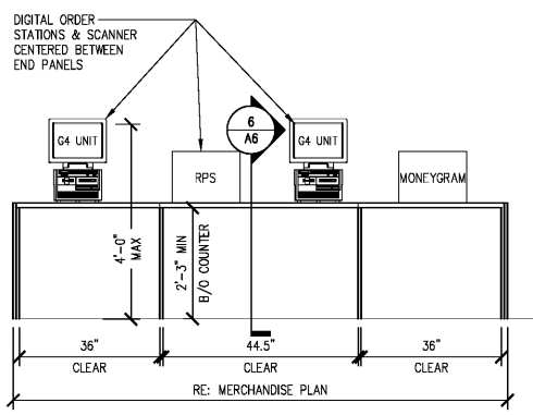
5 ADA PHOTOLAB COUNTER ELEVATION A6 SCALE: 1/2" = 1'-0"
