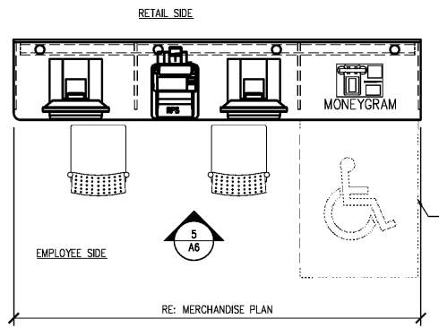
4 ADA PHOTOLAB COUNTER A6 SCALE: 1/2" = 1'-0"
