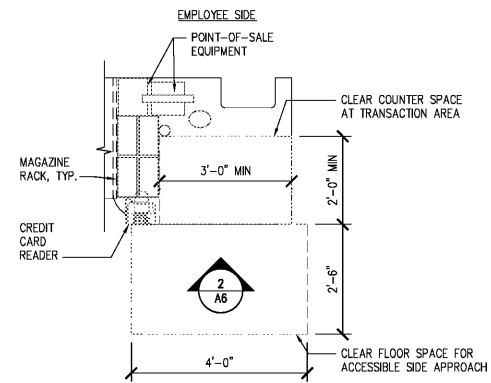
1 ADA FRONT CHECKOUT COUNTER A6 SCALE: 1/2" = 1'-0"
