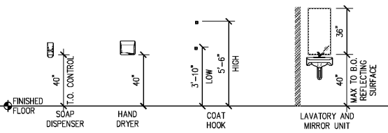
7 ACCESSIBLE MOUNTING HEIGHTS A6 SCALE: 1/4" = 1'-0"
