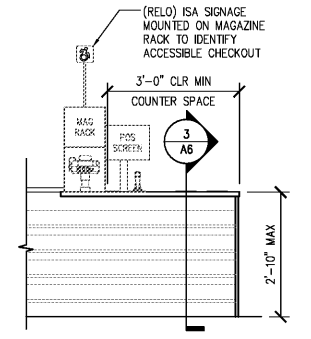
2 ADA FRONT CHECKOUT COUNTER ELEVATION A6 SCALE: 1/2" = 1'-0"
