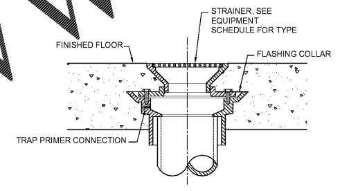
3 FLOOR DRAIN DETAIL P-301 NOT TO SCALE
