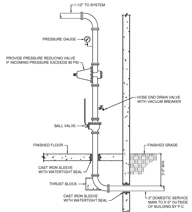
1 DOMESTIC SERVICE RISER DETAIL P-301 NOT TO SCALE
