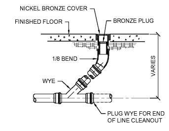
4 FLOOR CLEANOUT DETAIL P-301 NOT TO SCALE
