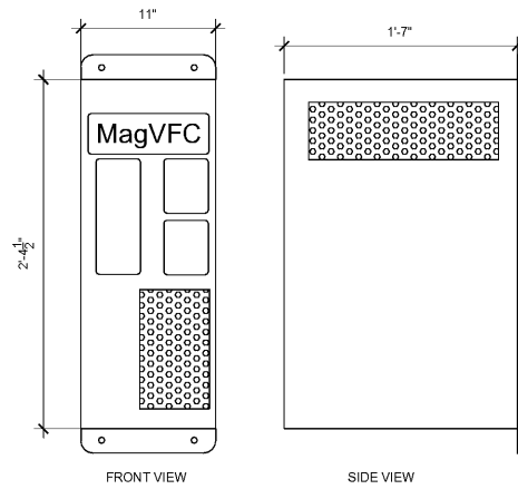
2 MAG VFC DETAIL NTS
