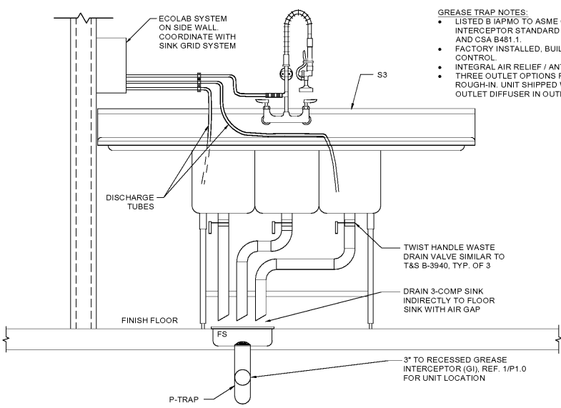
3 3-COMPARTMENT SINK DETAIL N.T.S.
