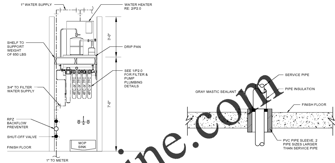
4 PLUMBING CONNECTION DETAIL 1/2" = 1'-0"
