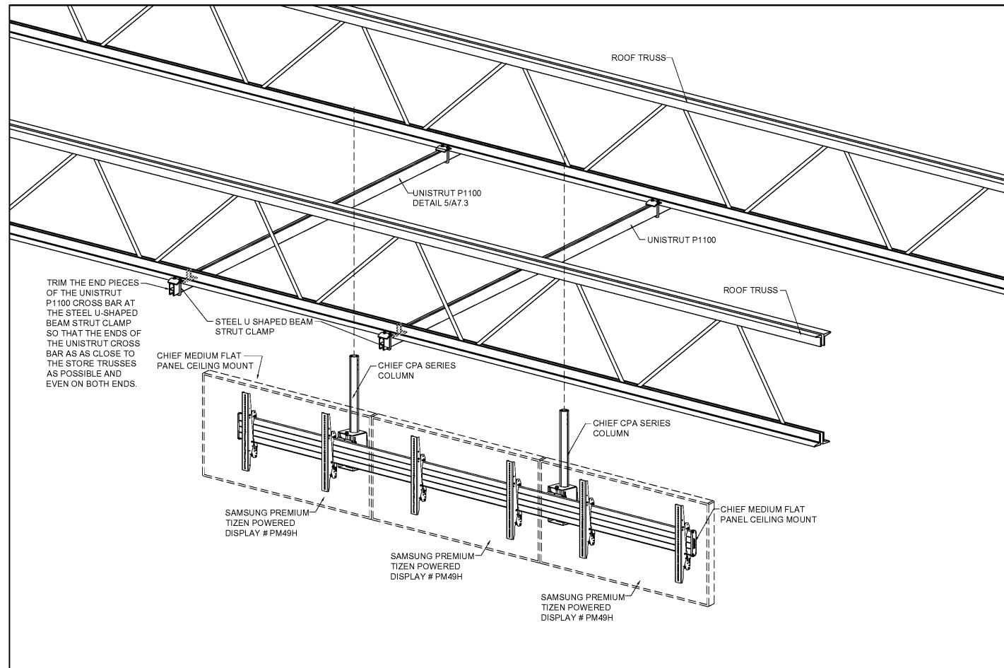
1 GENERAL THREE MENUBOARDS/PROMO SCREEN CEILING MOUNTING DETAIL 1/4" = 1'-0"
