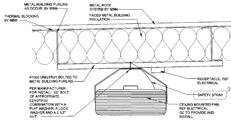
1 CEILING MOUNTED FAN SCALE: 1 1/2"=1'-0"
