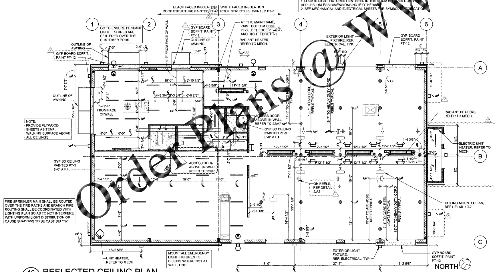
16 REFLECTED CEILING PLAN SCALE: 1/8"=1'-0"
