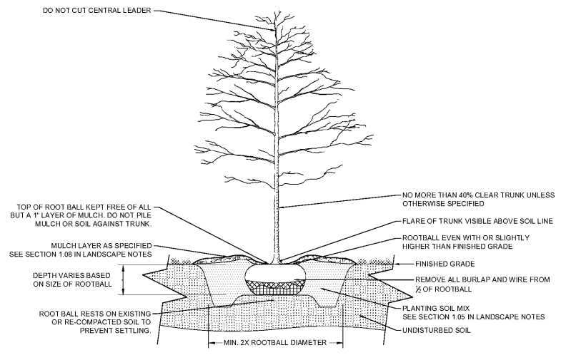
1 B&B TREE PLANTING NOT TO SCALE
