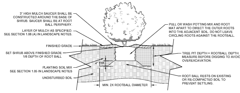
2 CONTAINER SHRUB PLANTING NOT TO SCALE
