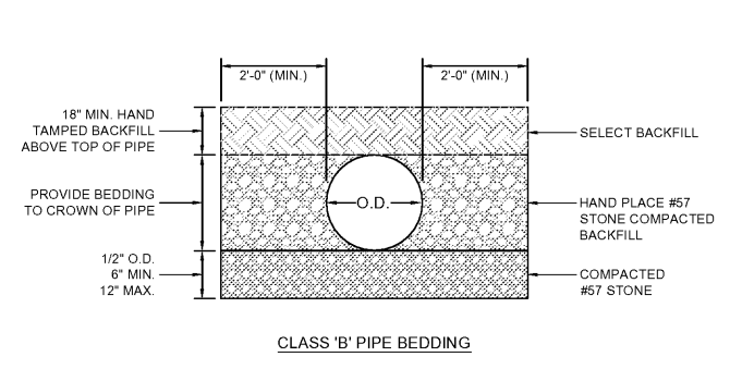
32 HDPE STORM DRAIN BEDDING DETAIL NOT TO SCALE
