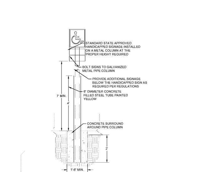
11 H'CAP SIGN DETAIL VAN ACCESSIBLE NOT TO SCALE
