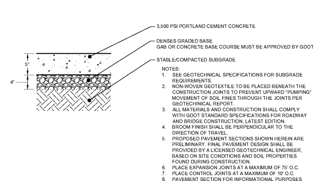
3 TYPICAL STANDARD CONCRETE PAVEMENT SECTION NOT TO SCALE
