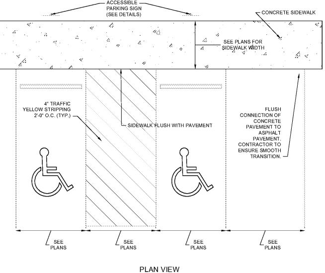
12 ADA CURB LAYOUT NOT TO SCALE
