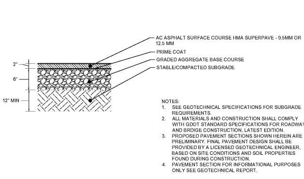
1 TYPICAL STANDARD DUTY ASPHALT PAVEMENT SECTION NOT TO SCALE
