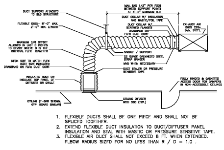
1 FLEXIBLE DUCT TAKEOFF DETAIL N.T.S.
