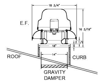
LOREN COOK E.F. 100C17DEC WITH GRAVITY DAMPER AND ROOF CURB ACCESSORY RCA-18 (REQUEST CURB TO MATCH ROOF PITCH)
