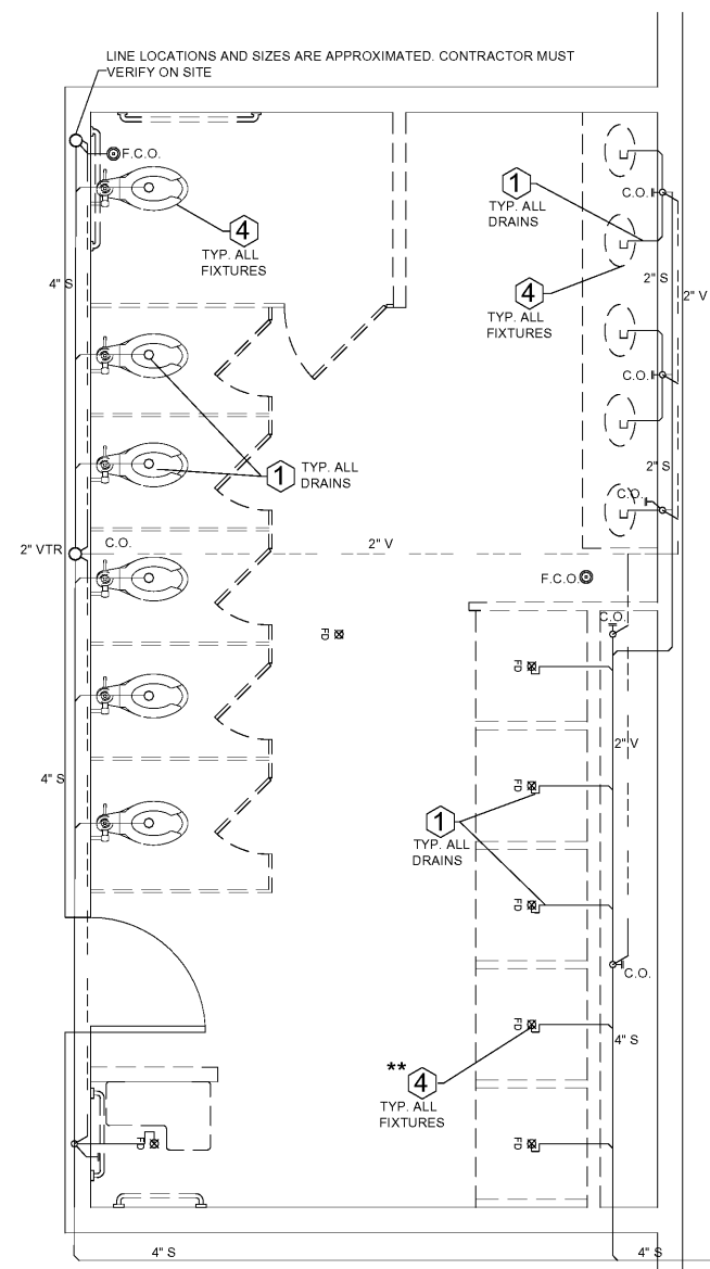
1 EXISTING BATHROOM 345 PLUMBING PLAN - BUILDING C SCALE: 1/2" = 1'-0"
