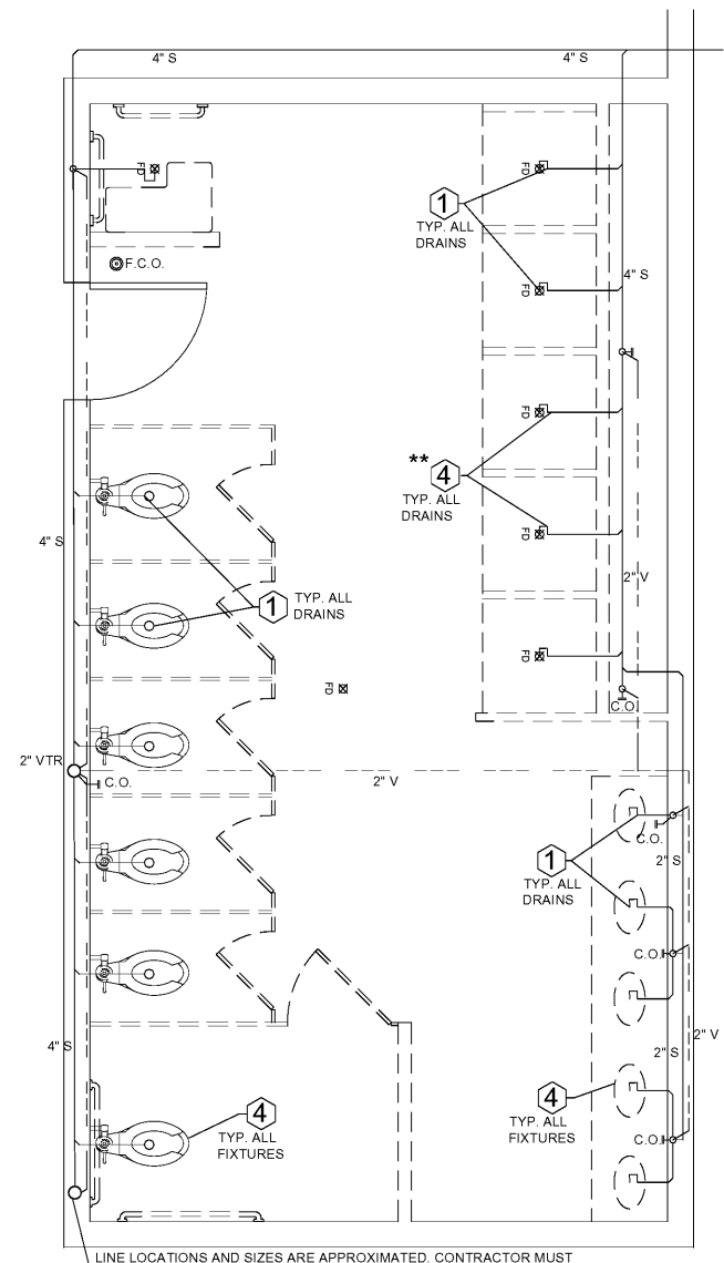
1 EXISTING BATHROOM 360 PLUMBING PLAN - BUILDING C SCALE: 1/2" = 1'-0"
