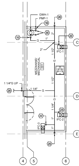
2 MEZZANINE POTABLE WATER AND GAS PIPING PLAN P-201 SCALE: 1/8" = 1'-0"
