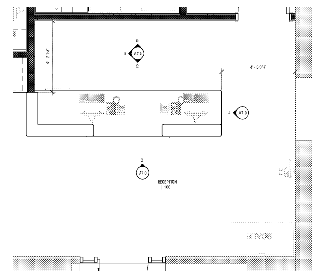
1 ENLARGED PLAN - RECEPTION A7.0 1/2" = 1'-0"
