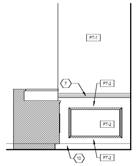
6 RECEPTION / 100 - WEST ELEVATION A7.0 1/2" = 1'-0"
