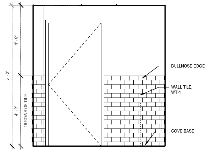
10 RESTROOM / 120 - SOUTH ELEVATION A6.0 1/2" = 1'-0"
