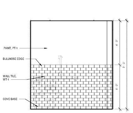
9 RESTROOM / 120 - EAST ELEVATION A6.0 1/2" = 1'-0"
