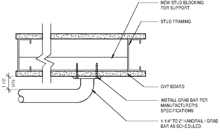
6 DETAIL - GRAB BAR WALL BLOCKING A6.0 3" = 1'-0"
