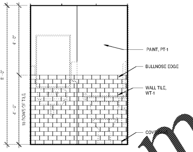
3 RESTROOM / 108 - EAST ELEVATION A6.0 1/2" = 1'-0"
