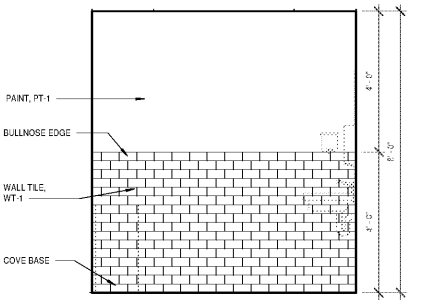
11 RESTROOM / 120 - WEST ELEVATION A6.0 1/2" = 1'-0"
