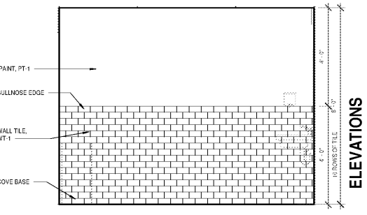
4 RESTROOM / 108 - NORTH ELEVATION A6.0 1/2" = 1'-0"
