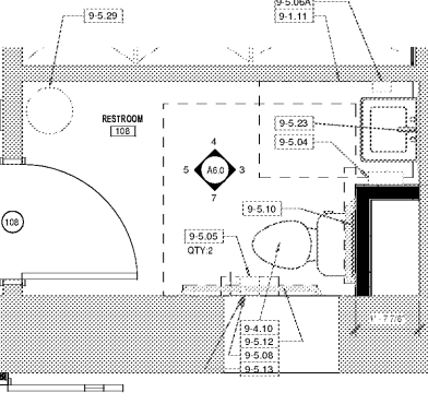
1 ENLARGED FLOOR PLAN - RESTROOM 108 A6.0 1/2" = 1'-0"
