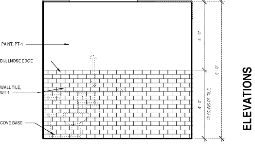
7 RESTROOM / 108 - SOUTH ELEVATION A6.0 1/2" = 1'-0"
