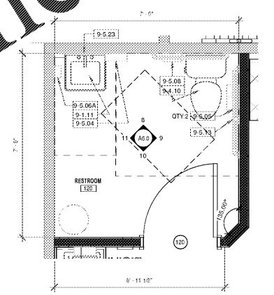
2 ENLARGED FLOOR PLAN - RESTROOM 120 A6.0 1/2" = 1'-0"
