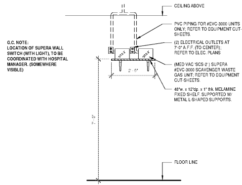
3 ELEVATION - MED. GAS EVACUATION PUMP STORAGE 1/2" = 1'-0"
