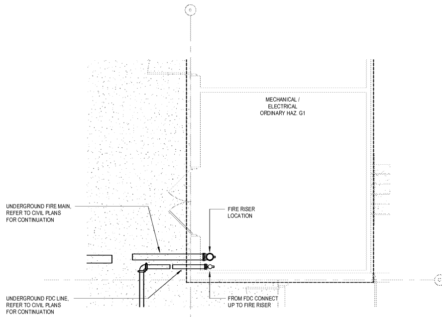
ENLARGED FIRE RISER ROOM - FIRE PROTECTION 1/4" = 1'-0" ②
